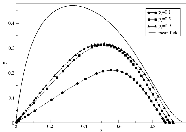
FIG. 2. The simulation results for the fraction of open channels y as a function of calcium density x using set 3 for p_a=0.1 , p_a=0.5 , and p_a=0.9 and lattice size L=40 . Comparison with mean field solution.
