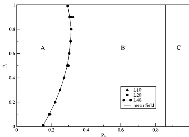
FIG. 5. The phase diagram for set 3 on the p_b - p_a plane, obtained from simulations for lattice sizes L=10, 20, 40 and mean field results. For simulations results region A represents the active states and regions B and C represent the absorbing states ( x=y=0 ). For mean field results the active states are represented by regions A and B and the absorbing states are represented by region C.
