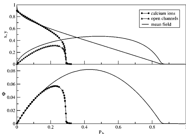
FIG. 3. The simulation results using set 3 for (a) the density of open channels y and of calcium ions x as a function of p_b for p_a = 0.5 (lattice size L=40 ) and (b) the flux \Phi as a function of p_b for p_a=0.5 (lattice sizes L=40 ). Comparison with mean field solution. We have p_b^c \approx 0.292 for simulations and p_b^c = 0.857 for mean field approximation.
