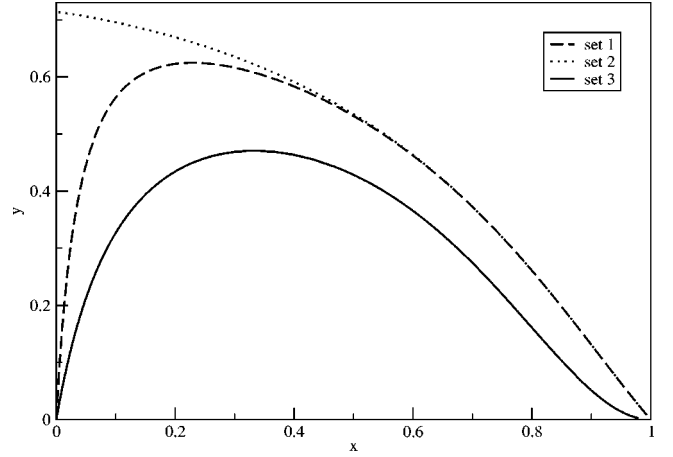
FIG. 1. The mean field results for the fraction of open channels y as a function of calcium density x . Sets 1, 2, and 3 are according to definition in Table I. Despite great similarities between sets 1 and 2, the absorbing state ( x=y=0 ) exists just in the first case. For set 3 the absorbing state is also present.
