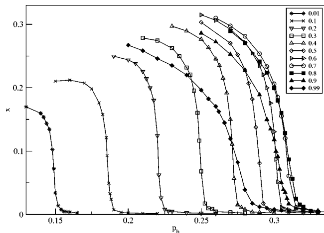
FIG. 4. The simulation results using set 3 for calcium density x as a function of p_b for several values of p_a (indicated in the figure). Lattice size L=40 .
